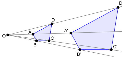
Figure 17.1: A homothety with center O and ratio k = 2.5
