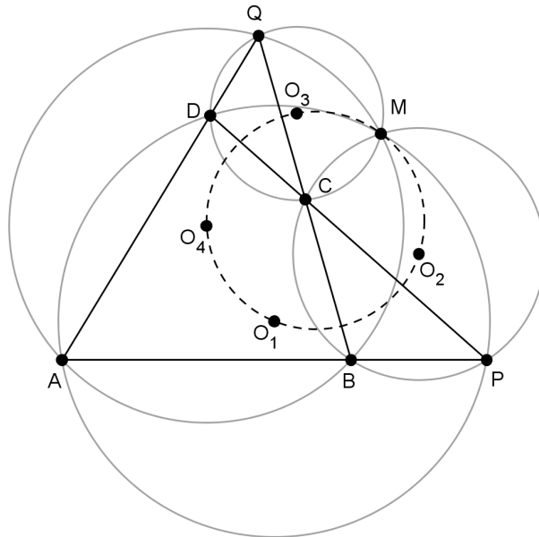
Figure 19.1: The circumcircles of \triangle ABQ , \triangle BCP , \triangle CDQ and \triangle DAP pass through the Miquel point M . Their circumcenters and M are concyclic.
