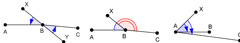
Figure 8.1: Three collinearity configurations
