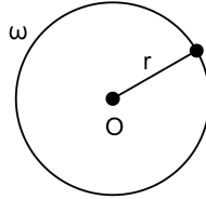
Figure 5.1: Circle \omega with center O and radius r .
