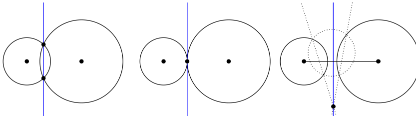
Figure 14.1: Radical axis of two circles
