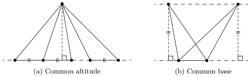
Figure 3.1: Triangles with equal area
