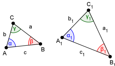
Figure 4.1: Similar triangles.
