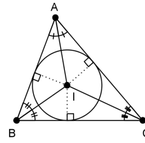
(b) Incenter
