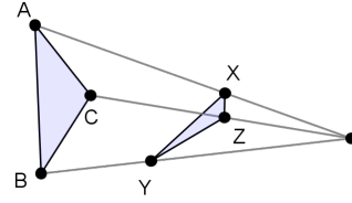
(b) Perspective from a point.
