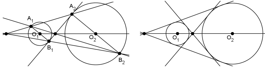
Figure 17.2: Internal and external homothetic center of two circles.
